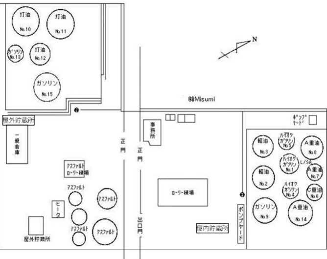
図5 (株) Misumi Yatsu branch configuration diagram
